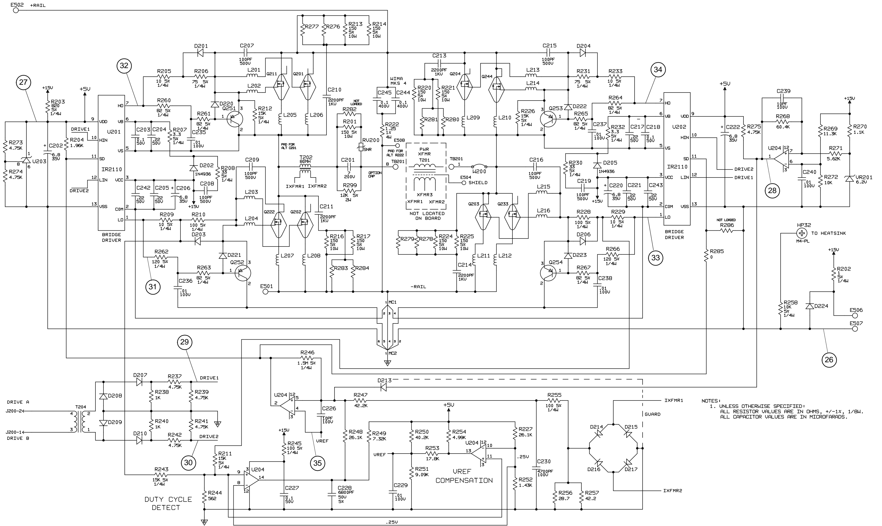
Figure 6-8. A3 FET Board Schematic Diagram
